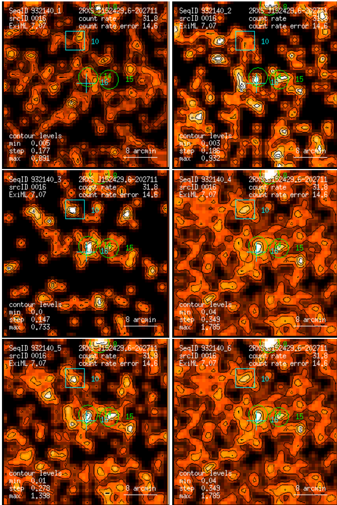
Figure 16: RASS 932140: detection 0016: band rate images, Gaussian filter: (1) PSPC channels 11 – 41, (2) 52 – 90, (3) 91 – 201, (4) 11 – 235, (5) 52 – 201, (6) 11 – 201. Broad band rates in counts/ks. Band rate contour levels in counts/ks/arcmin 2 .
