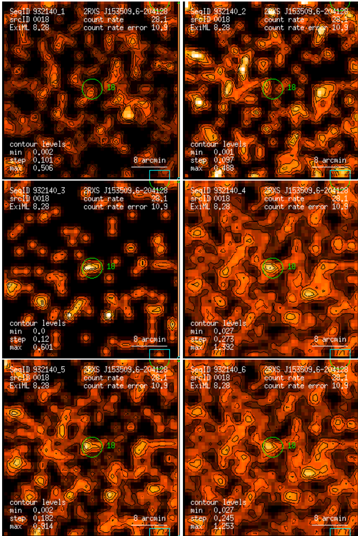
Figure 18: RASS 932140: detection 0018: band rate images, Gaussian filter: (1) PSPC channels 11 – 41, (2) 52 – 90, (3) 91 – 201, (4) 11 – 235, (5) 52 – 201, (6) 11 – 201. Broad band rates in counts/ks. Band rate contour levels in counts/ks/arcmin 2 .
