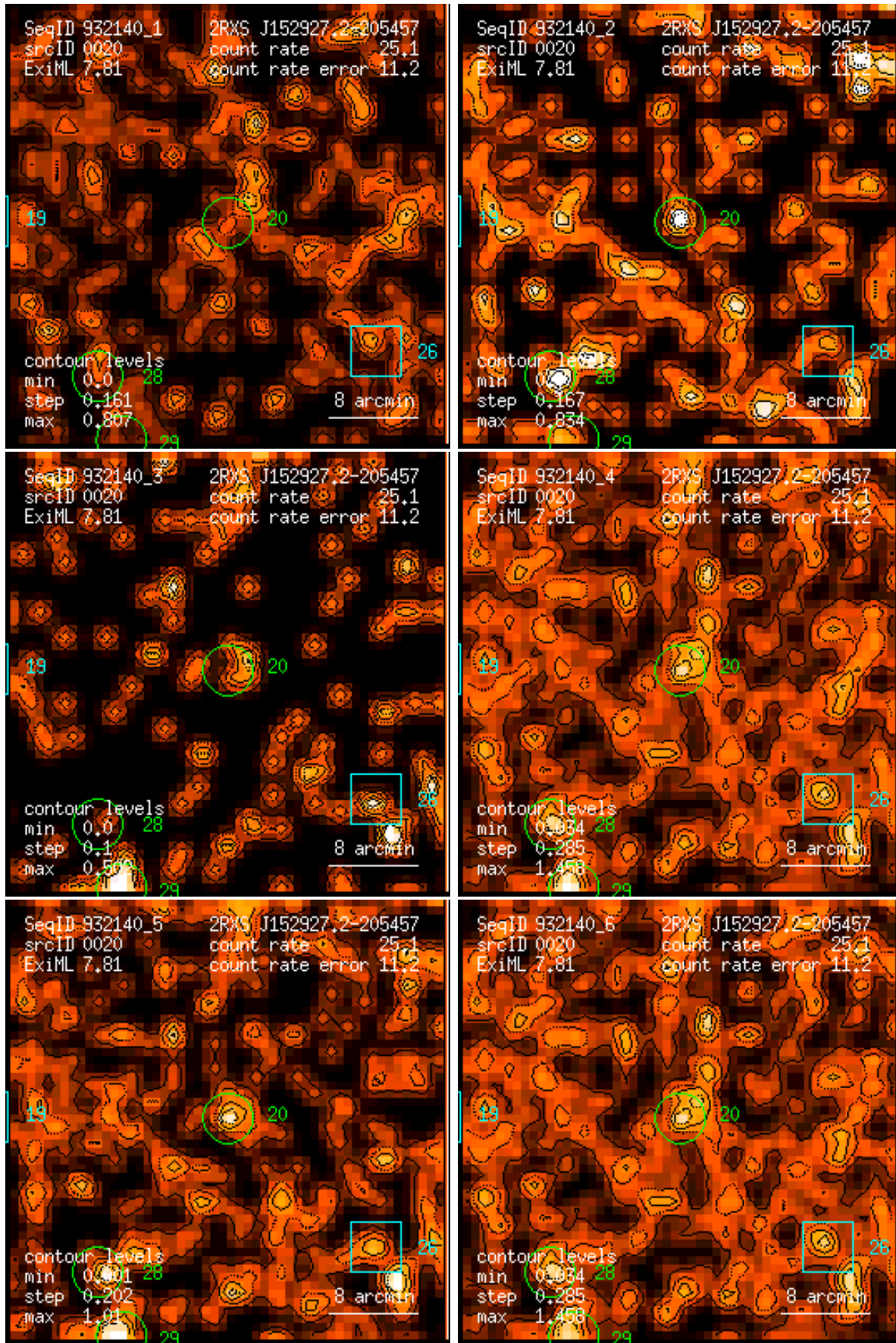
Figure 20: RASS 932140: detection 0020: band rate images, Gaussian filter: (1) PSPC channels 11 – 41, (2) 52 – 90, (3) 91 – 201, (4) 11 – 235, (5) 52 – 201, (6) 11 – 201. Broad band rates in counts/ks. Band rate contour levels in counts/ks/arcmin 2 .
