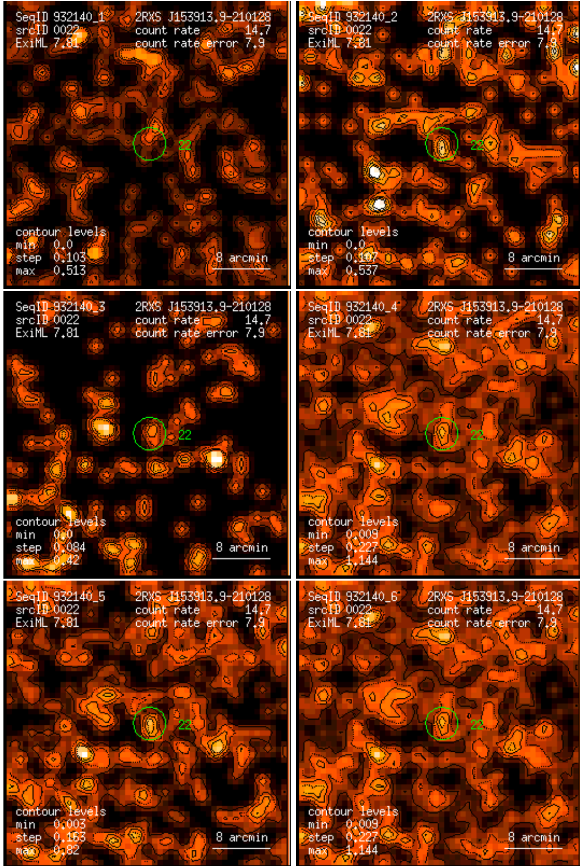
Figure 22: RASS 932140: detection 0022: band rate images, Gaussian filter: (1) PSPC channels 11 – 41, (2) 52 – 90, (3) 91 – 201, (4) 11 – 235, (5) 52 – 201, (6) 11 – 201. Broad band rates in counts/ks. Band rate contour levels in counts/ks/arcmin 2 .
