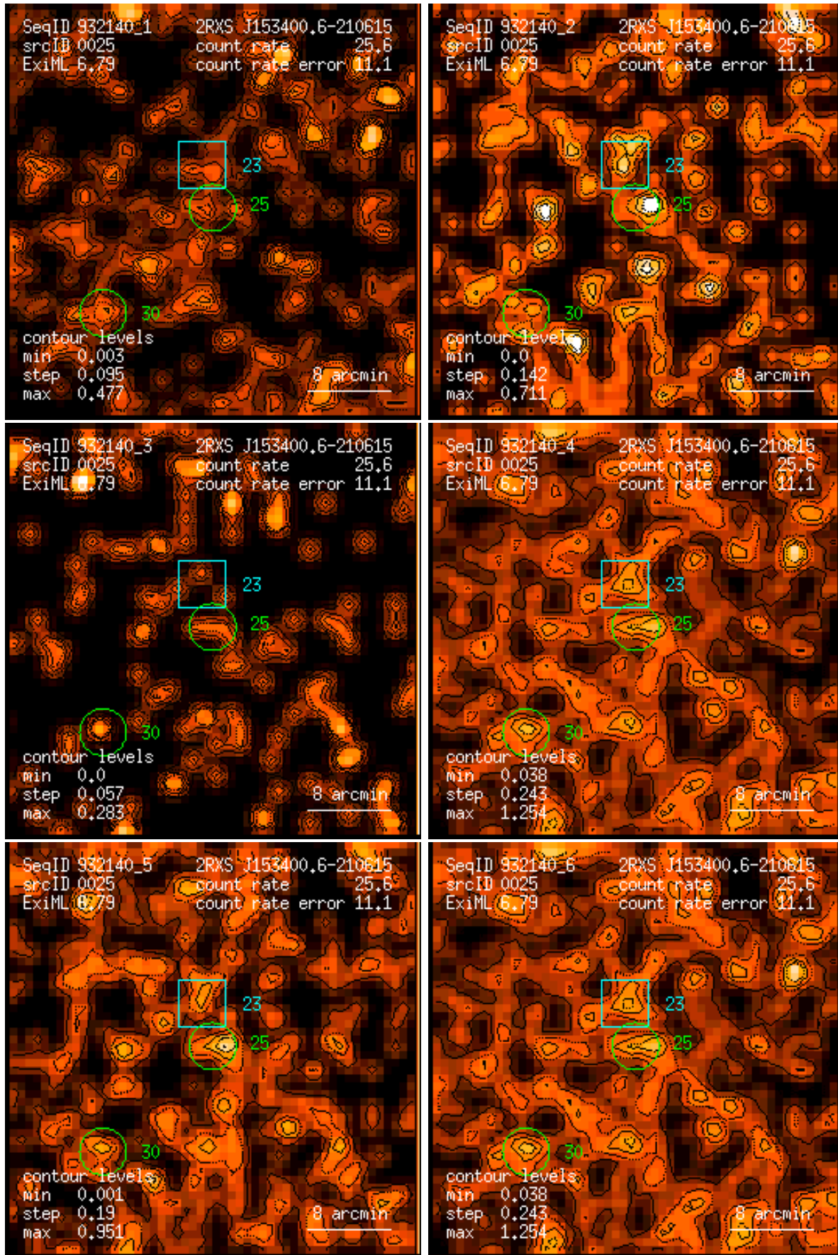
Figure 25: RASS 932140: detection 0025: band rate images, Gaussian filter: (1) PSPC channels 11 – 41, (2) 52 – 90, (3) 91 – 201, (4) 11 – 235, (5) 52 – 201, (6) 11 – 201. Broad band rates in counts/ks. Band rate contour levels in counts/ks/arcmin 2 .
