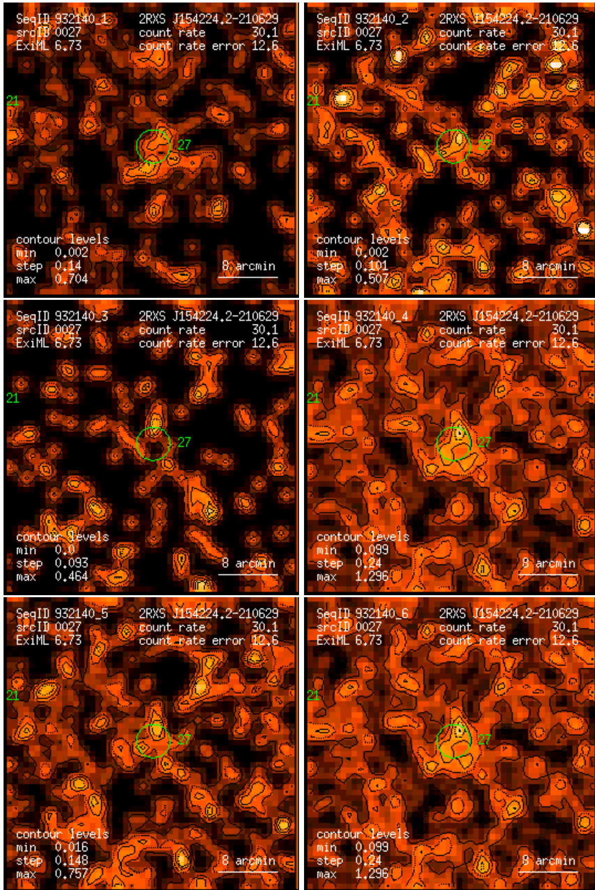
Figure 27: RASS 932140: detection 0027: band rate images, Gaussian filter: (1) PSPC channels 11 – 41, (2) 52 – 90, (3) 91 – 201, (4) 11 – 235, (5) 52 – 201, (6) 11 – 201. Broad band rates in counts/ks. Band rate contour levels in counts/ks/arcmin 2 .
