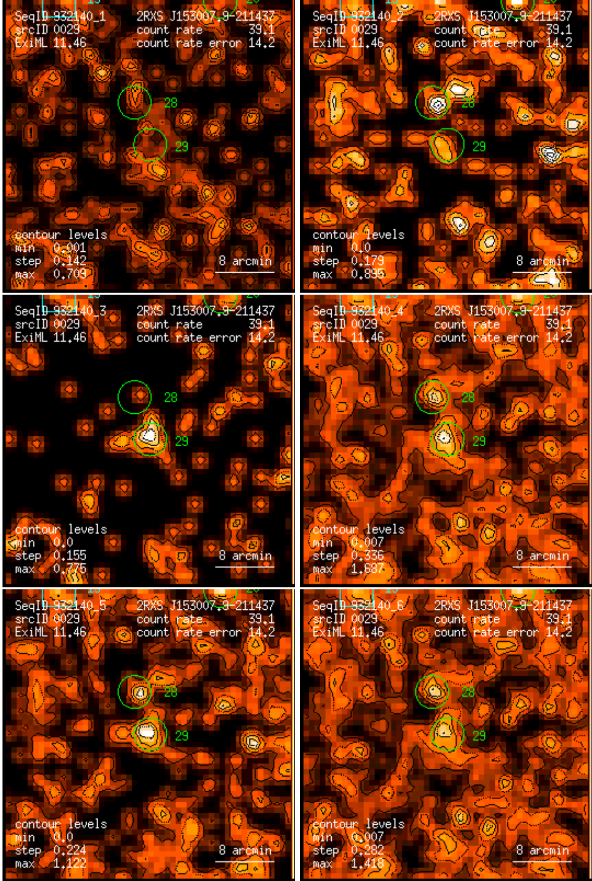
Figure 29: RASS 932140: detection 0029: band rate images, Gaussian filter: (1) PSPC channels 11 – 41, (2) 52 – 90, (3) 91 – 201, (4) 11 – 235, (5) 52 – 201, (6) 11 – 201. Broad band rates in counts/ks. Band rate contour levels in counts/ks/arcmin 2 .
