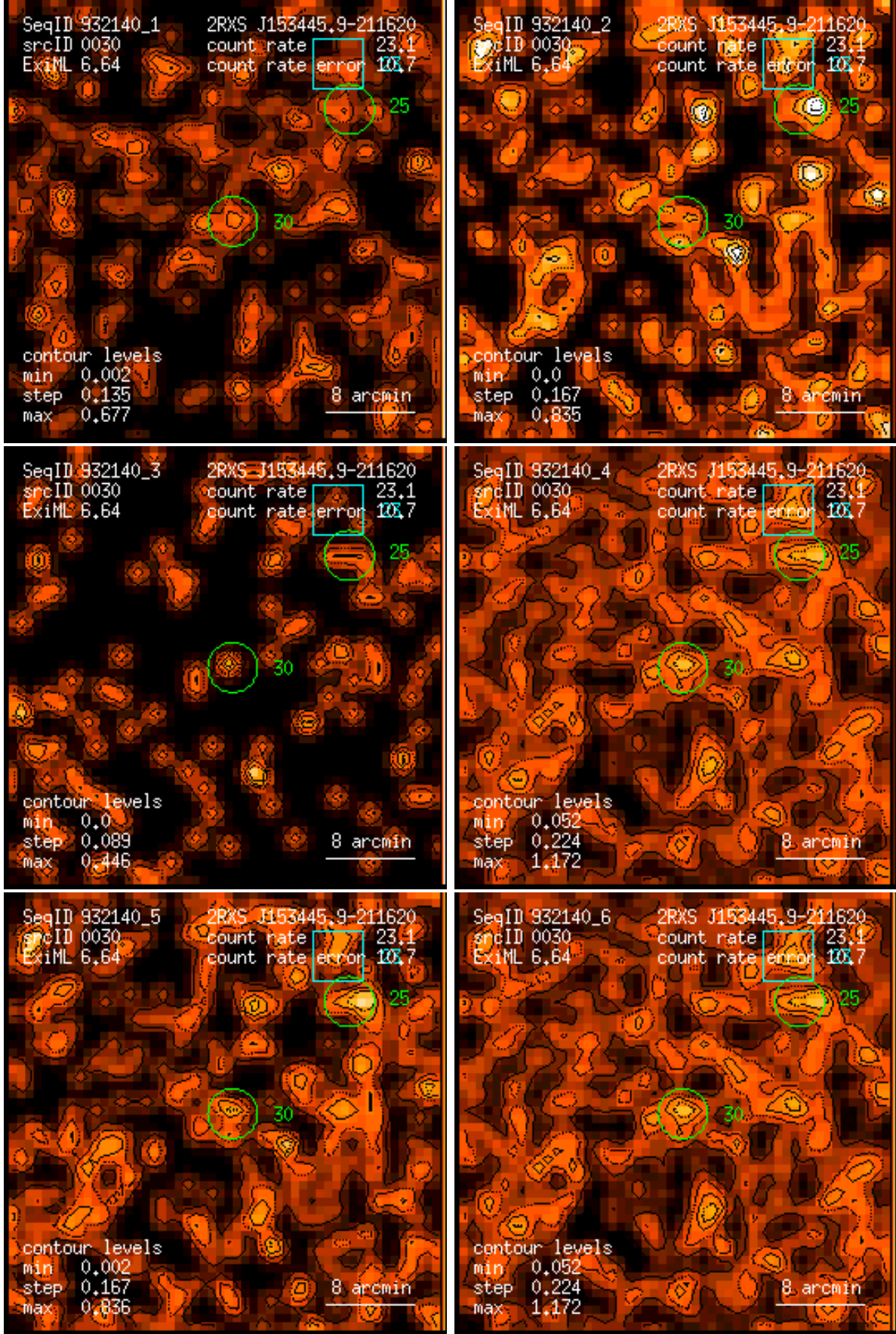
Figure 30: RASS 932140: detection 0030: band rate images, Gaussian filter: (1) PSPC channels 11 – 41, (2) 52 – 90, (3) 91 – 201, (4) 11 – 235, (5) 52 – 201, (6) 11 – 201. Broad band rates in counts/ks. Band rate contour levels in counts/ks/arcmin 2 .
