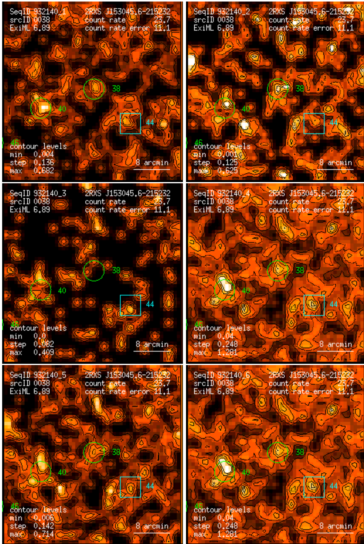
Figure 38: RASS 932140: detection 0038: band rate images, Gaussian filter: (1) PSPC channels 11 – 41, (2) 52 – 90, (3) 91 – 201, (4) 11 – 235, (5) 52 – 201, (6) 11 – 201. Broad band rates in counts/ks. Band rate contour levels in counts/ks/arcmin 2 .
