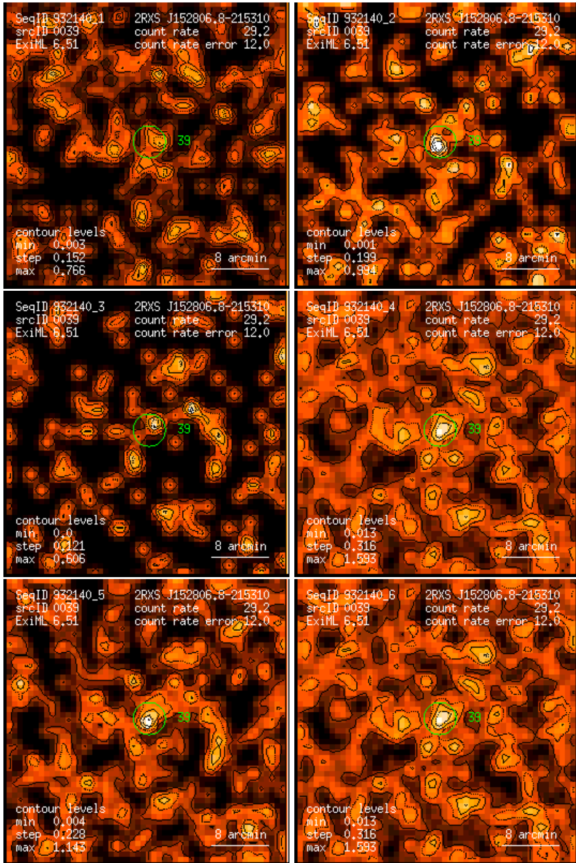
Figure 39: RASS 932140: detection 0039: band rate images, Gaussian filter: (1) PSPC channels 11 – 41, (2) 52 – 90, (3) 91 – 201, (4) 11 – 235, (5) 52 – 201, (6) 11 – 201. Broad band rates in counts/ks. Band rate contour levels in counts/ks/arcmin 2 .
