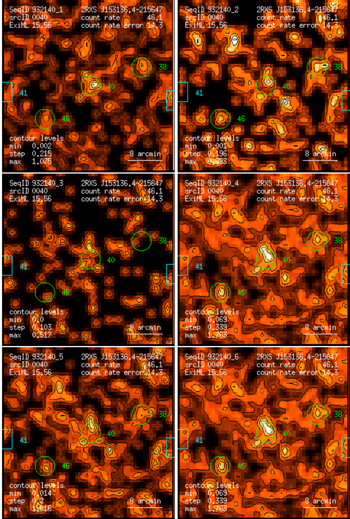
Figure 40: RASS 932140: detection 0040: band rate images, Gaussian filter: (1) PSPC channels 11 – 41, (2) 52 – 90, (3) 91 – 201, (4) 11 – 235, (5) 52 – 201, (6) 11 – 201. Broad band rates in counts/ks. Band rate contour levels in counts/ks/arcmin 2 .
