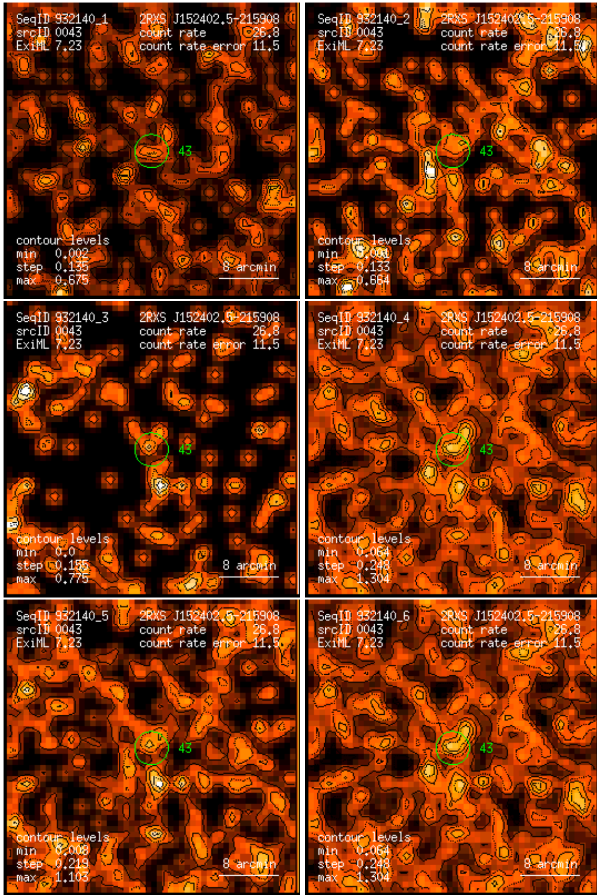
Figure 43: RASS 932140: detection 0043: band rate images, Gaussian filter: (1) PSPC channels 11 – 41, (2) 52 – 90, (3) 91 – 201, (4) 11 – 235, (5) 52 – 201, (6) 11 – 201. Broad band rates in counts/ks. Band rate contour levels in counts/ks/arcmin 2 .
