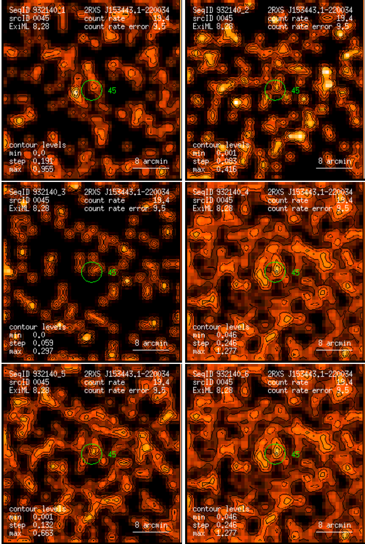
Figure 45: RASS 932140: detection 0045: band rate images, Gaussian filter: (1) PSPC channels 11 – 41, (2) 52 – 90, (3) 91 – 201, (4) 11 – 235, (5) 52 – 201, (6) 11 – 201. Broad band rates in counts/ks. Band rate contour levels in counts/ks/arcmin 2 .
