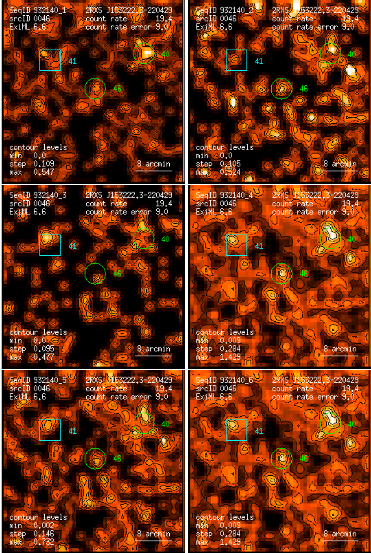
Figure 46: RASS 932140: detection 0046: band rate images, Gaussian filter: (1) PSPC channels 11 – 41, (2) 52 – 90, (3) 91 – 201, (4) 11 – 235, (5) 52 – 201, (6) 11 – 201. Broad band rates in counts/ks. Band rate contour levels in counts/ks/arcmin 2 .
