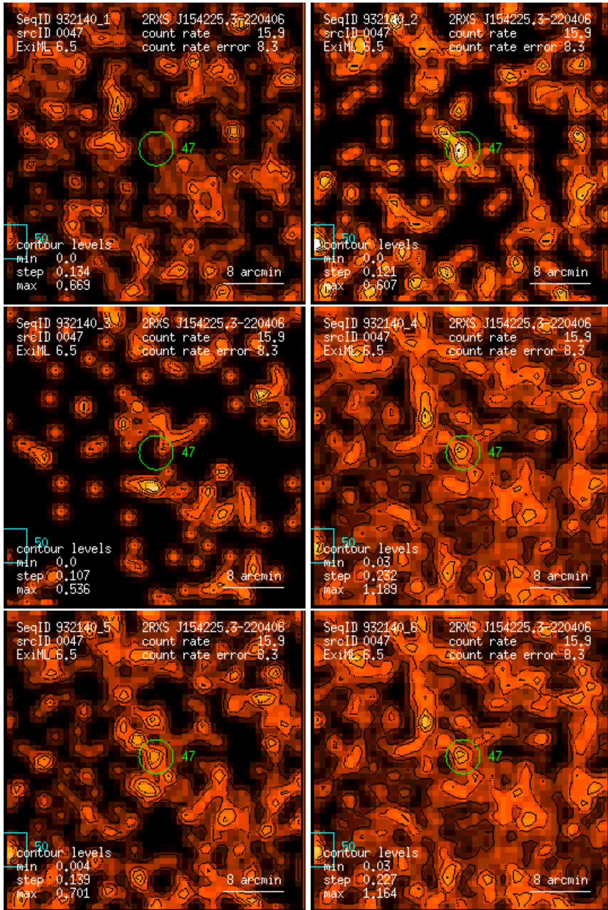
Figure 47: RASS 932140: detection 0047: band rate images, Gaussian filter: (1) PSPC channels 11 – 41, (2) 52 – 90, (3) 91 – 201, (4) 11 – 235, (5) 52 – 201, (6) 11 – 201. Broad band rates in counts/ks. Band rate contour levels in counts/ks/arcmin 2 .
