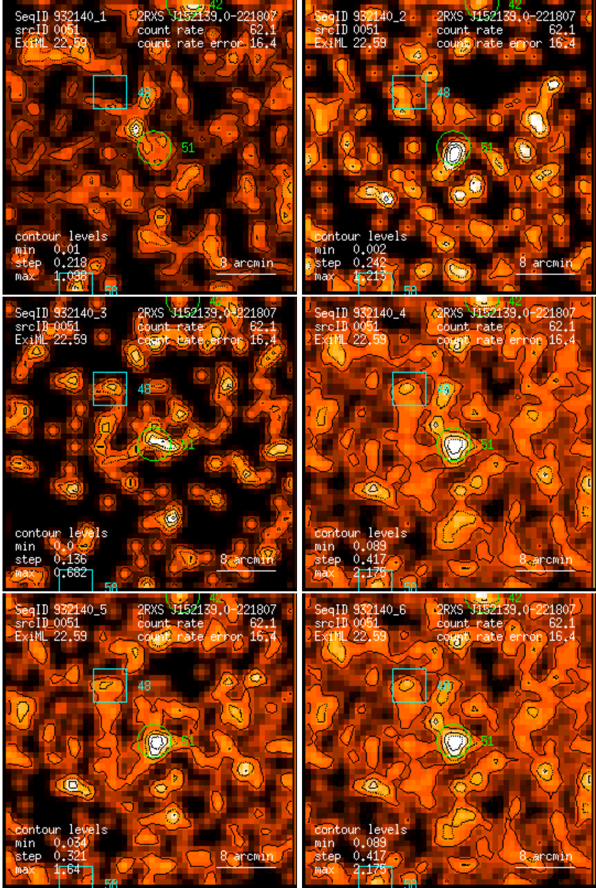
Figure 51: RASS 932140: detection 0051: band rate images, Gaussian filter: (1) PSPC channels 11 – 41, (2) 52 – 90, (3) 91 – 201, (4) 11 – 235, (5) 52 – 201, (6) 11 – 201. Broad band rates in counts/ks. Band rate contour levels in counts/ks/arcmin 2 .
