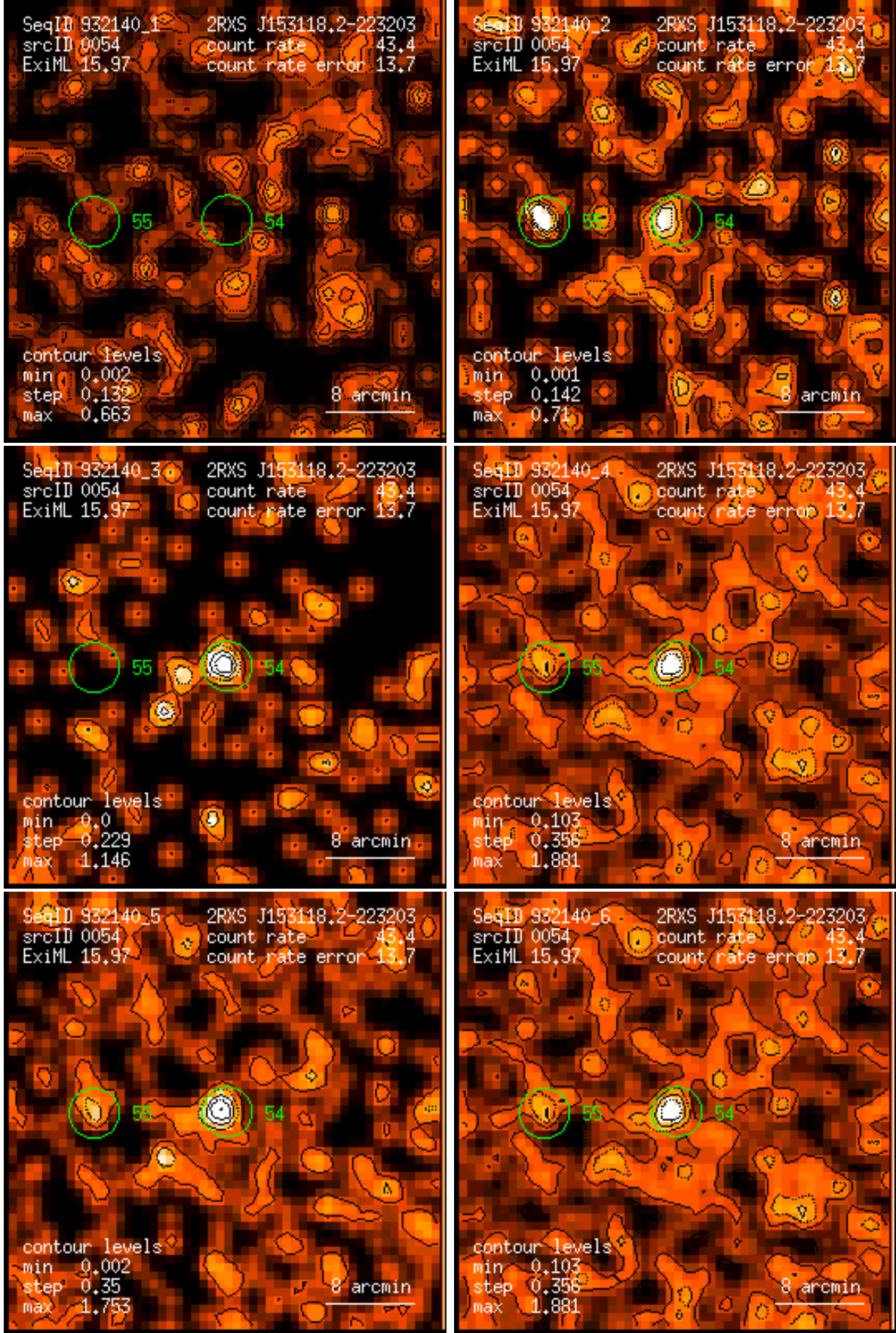
Figure 54: RASS 932140: detection 0054: band rate images, Gaussian filter: (1) PSPC channels 11 – 41, (2) 52 – 90, (3) 91 – 201, (4) 11 – 235, (5) 52 – 201, (6) 11 – 201. Broad band rates in counts/ks. Band rate contour levels in counts/ks/arcmin 2 .
