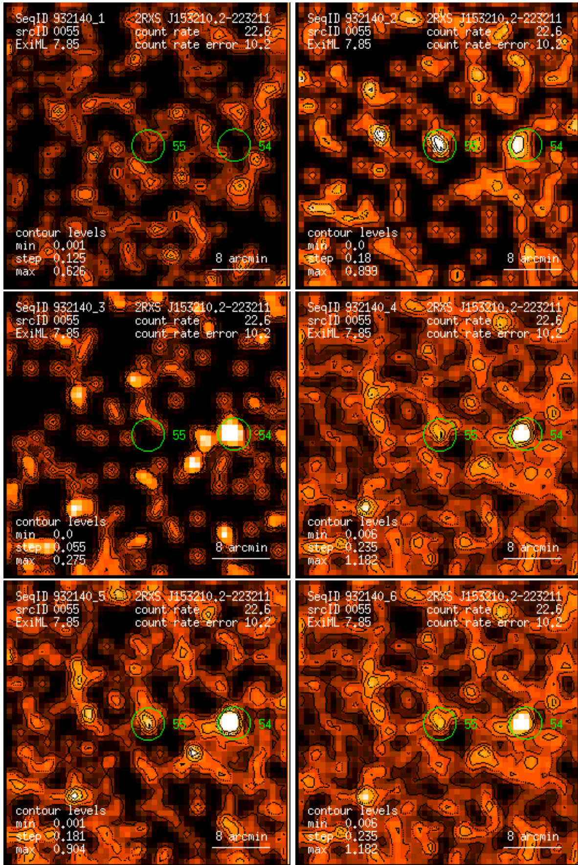
Figure 55: RASS 932140: detection 0055: band rate images, Gaussian filter: (1) PSPC channels 11 – 41, (2) 52 – 90, (3) 91 – 201, (4) 11 – 235, (5) 52 – 201, (6) 11 – 201. Broad band rates in counts/ks. Band rate contour levels in counts/ks/arcmin 2 .
