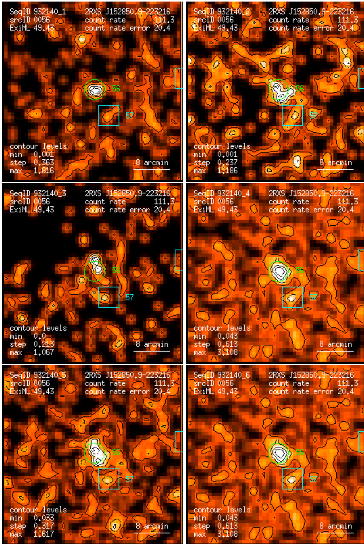
Figure 56: RASS 932140: detection 0056: band rate images, Gaussian filter: (1) PSPC channels 11 – 41, (2) 52 – 90, (3) 91 – 201, (4) 11 – 235, (5) 52 – 201, (6) 11 – 201. Broad band rates in counts/ks. Band rate contour levels in counts/ks/arcmin 2 .
