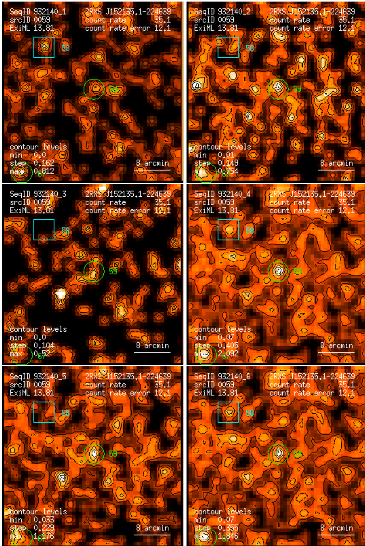
Figure 59: RASS 932140: detection 0059: band rate images, Gaussian filter: (1) PSPC channels 11 – 41, (2) 52 – 90, (3) 91 – 201, (4) 11 – 235, (5) 52 – 201, (6) 11 – 201. Broad band rates in counts/ks. Band rate contour levels in counts/ks/arcmin 2 .
