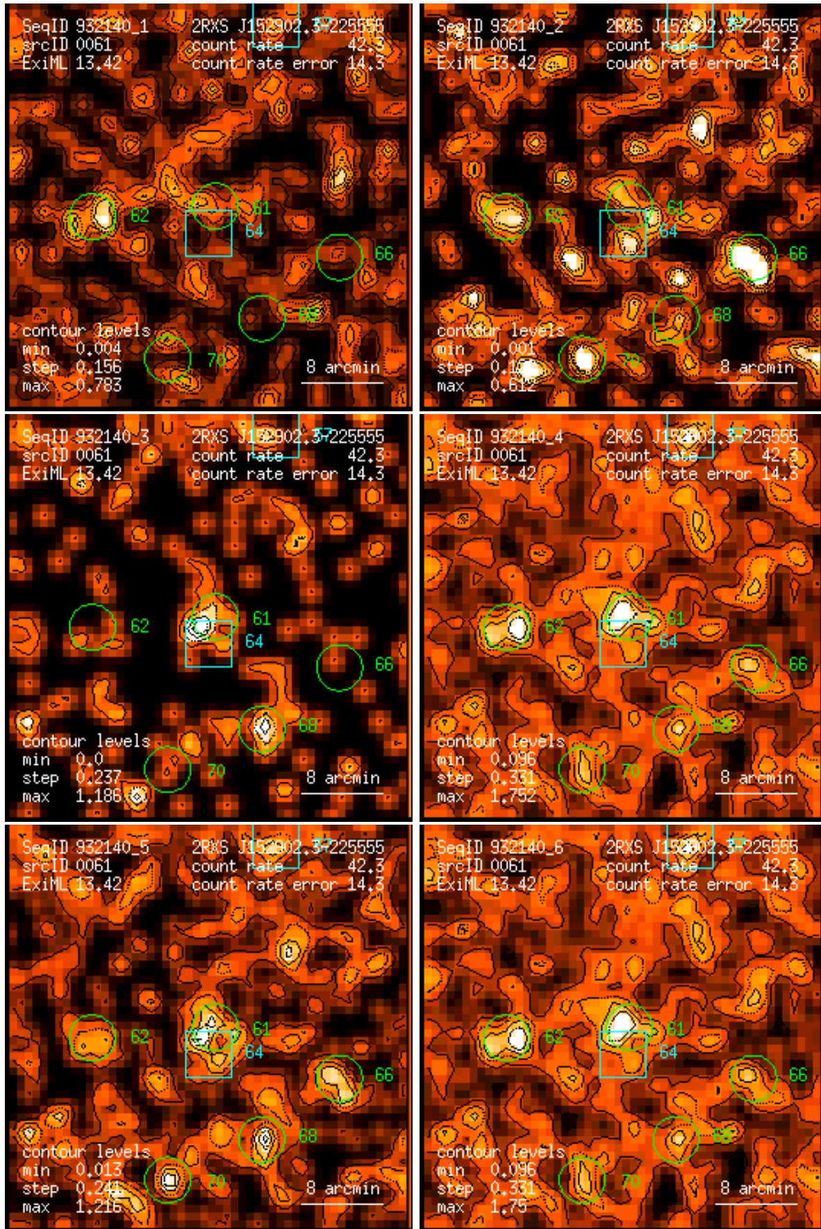
Figure 61: RASS 932140: detection 0061: band rate images, Gaussian filter: (1) PSPC channels 11 – 41, (2) 52 – 90, (3) 91 – 201, (4) 11 – 235, (5) 52 – 201, (6) 11 – 201. Broad band rates in counts/ks. Band rate contour levels in counts/ks/arcmin 2 .
