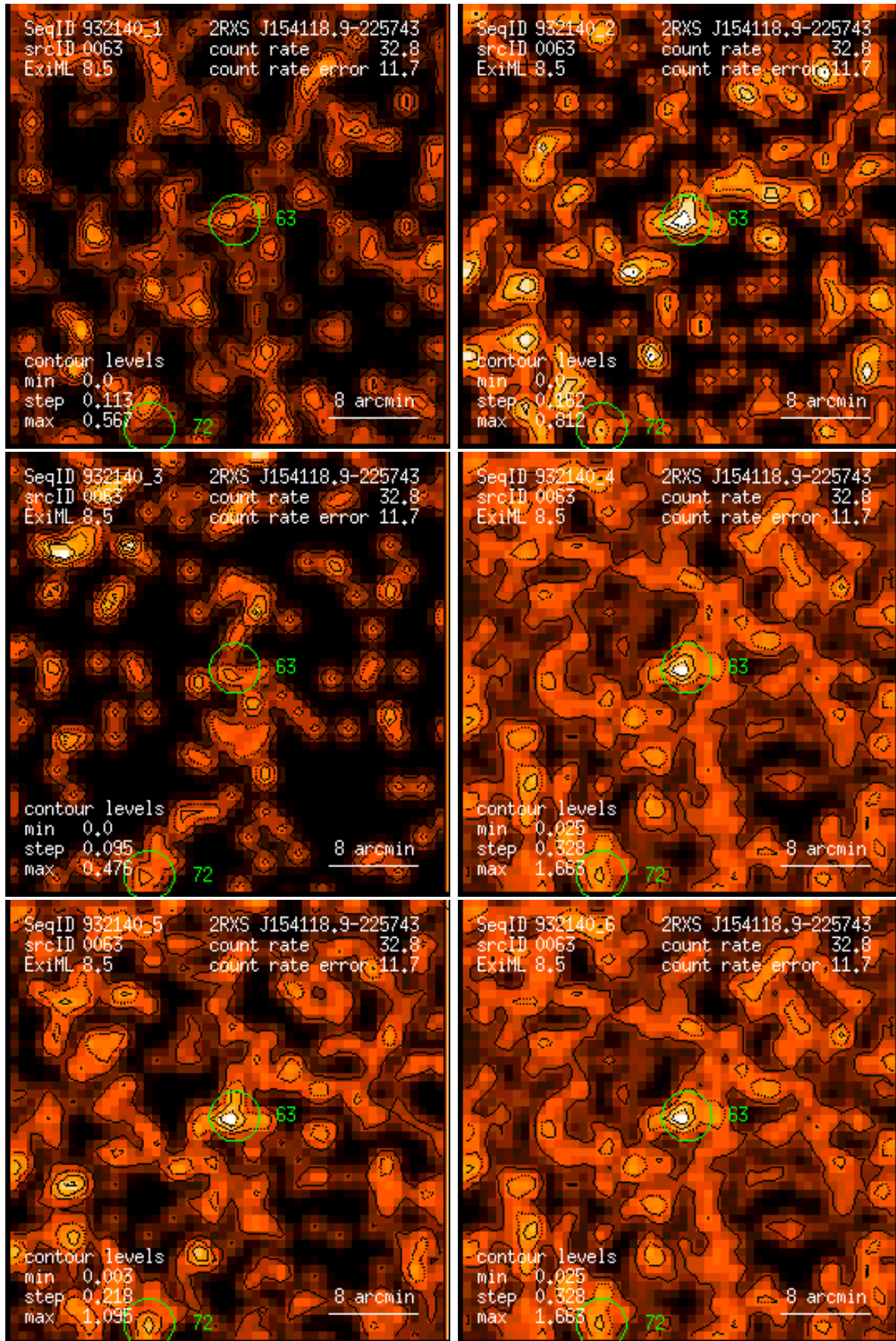
Figure 63: RASS 932140: detection 0063: band rate images, Gaussian filter: (1) PSPC channels 11 – 41, (2) 52 – 90, (3) 91 – 201, (4) 11 – 235, (5) 52 – 201, (6) 11 – 201. Broad band rates in counts/ks. Band rate contour levels in counts/ks/arcmin 2 .
