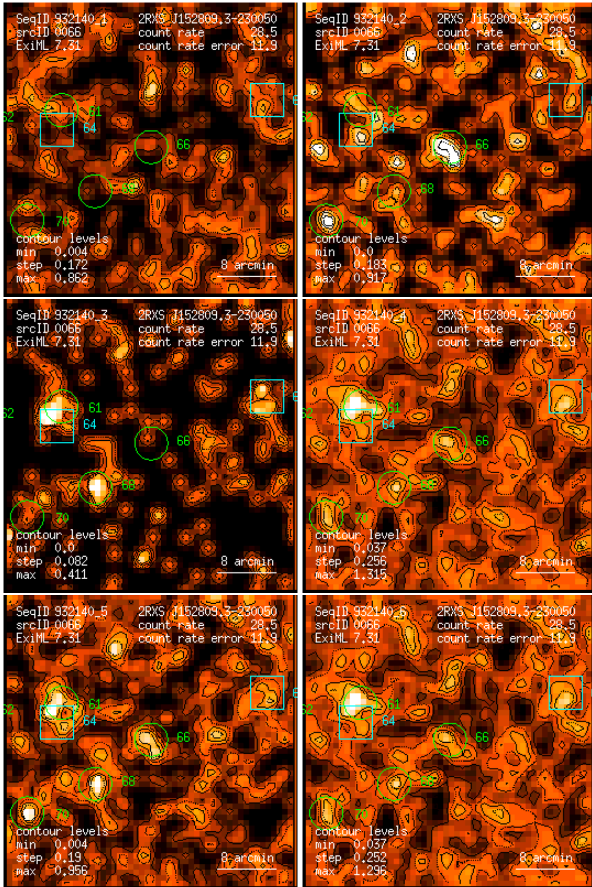
Figure 66: RASS 932140: detection 0066: band rate images, Gaussian filter: (1) PSPC channels 11 – 41, (2) 52 – 90, (3) 91 – 201, (4) 11 – 235, (5) 52 – 201, (6) 11 – 201. Broad band rates in counts/ks. Band rate contour levels in counts/ks/arcmin 2 .
