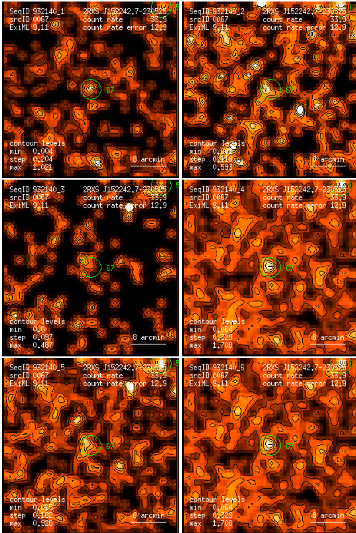
Figure 67: RASS 932140: detection 0067: band rate images, Gaussian filter: (1) PSPC channels 11 – 41, (2) 52 – 90, (3) 91 – 201, (4) 11 – 235, (5) 52 – 201, (6) 11 – 201. Broad band rates in counts/ks. Band rate contour levels in counts/ks/arcmin 2 .
