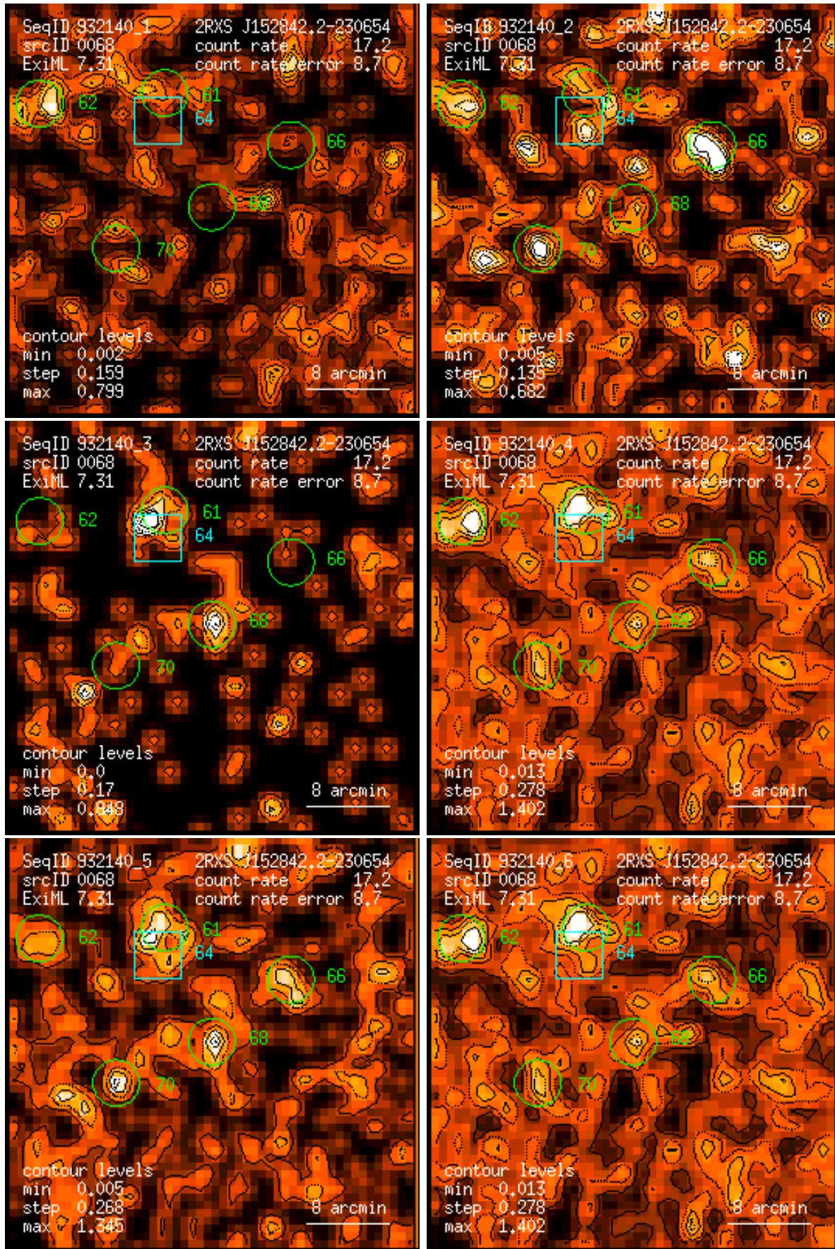
Figure 68: RASS 932140: detection 0068: band rate images, Gaussian filter: (1) PSPC channels 11 – 41, (2) 52 – 90, (3) 91 – 201, (4) 11 – 235, (5) 52 – 201, (6) 11 – 201. Broad band rates in counts/ks. Band rate contour levels in counts/ks/arcmin 2 .
