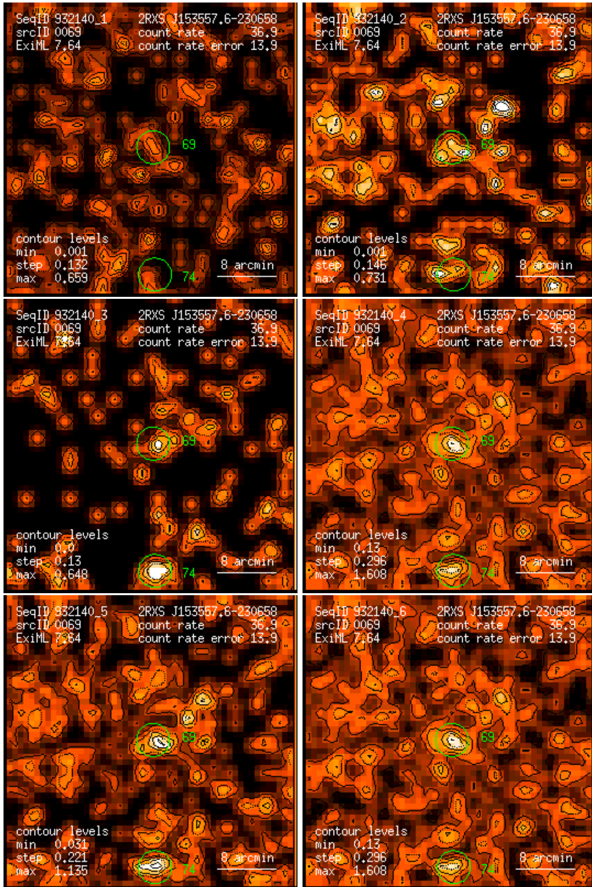
Figure 69: RASS 932140: detection 0069: band rate images, Gaussian filter: (1) PSPC channels 11 – 41, (2) 52 – 90, (3) 91 – 201, (4) 11 – 235, (5) 52 – 201, (6) 11 – 201. Broad band rates in counts/ks. Band rate contour levels in counts/ks/arcmin 2 .
