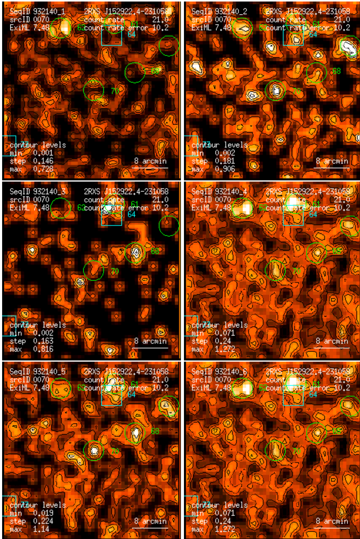
Figure 70: RASS 932140: detection 0070: band rate images, Gaussian filter: (1) PSPC channels 11 – 41, (2) 52 – 90, (3) 91 – 201, (4) 11 – 235, (5) 52 – 201, (6) 11 – 201. Broad band rates in counts/ks. Band rate contour levels in counts/ks/arcmin 2 .
