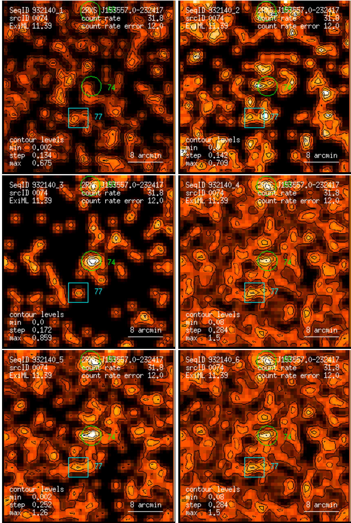
Figure 74: RASS 932140: detection 0074: band rate images, Gaussian filter: (1) PSPC channels 11 – 41, (2) 52 – 90, (3) 91 – 201, (4) 11 – 235, (5) 52 – 201, (6) 11 – 201. Broad band rates in counts/ks. Band rate contour levels in counts/ks/arcmin 2 .
