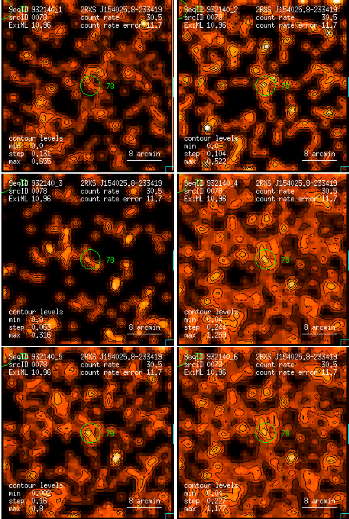
Figure 78: RASS 932140: detection 0078: band rate images, Gaussian filter: (1) PSPC channels 11 – 41, (2) 52 – 90, (3) 91 – 201, (4) 11 – 235, (5) 52 – 201, (6) 11 – 201. Broad band rates in counts/ks. Band rate contour levels in counts/ks/arcmin 2 .
