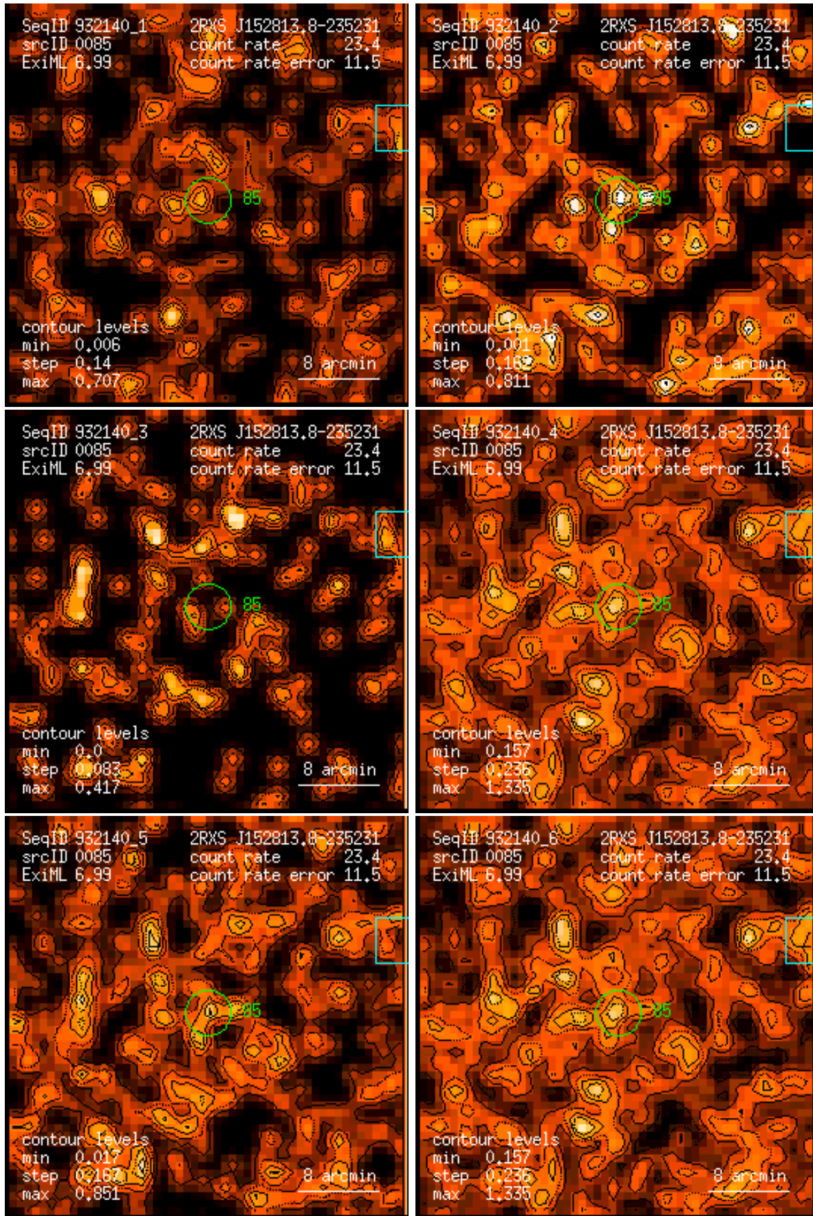
Figure 85: RASS 932140: detection 0085: band rate images, Gaussian filter: (1) PSPC channels 11 – 41, (2) 52 – 90, (3) 91 – 201, (4) 11 – 235, (5) 52 – 201, (6) 11 – 201. Broad band rates in counts/ks. Band rate contour levels in counts/ks/arcmin 2 .
