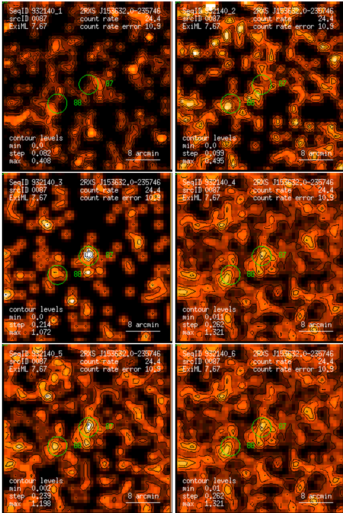
Figure 87: RASS 932140: detection 0087: band rate images, Gaussian filter: (1) PSPC channels 11 – 41, (2) 52 – 90, (3) 91 – 201, (4) 11 – 235, (5) 52 – 201, (6) 11 – 201. Broad band rates in counts/ks. Band rate contour levels in counts/ks/arcmin 2 .
