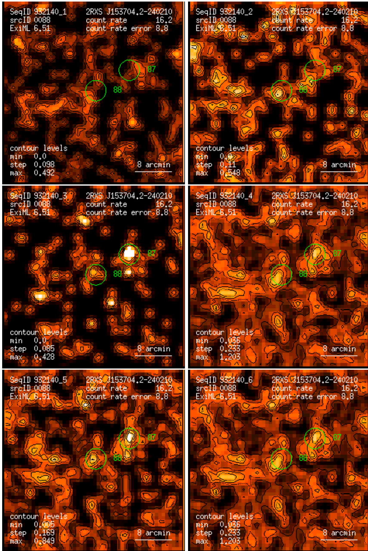
Figure 88: RASS 932140: detection 0088: band rate images, Gaussian filter: (1) PSPC channels 11 – 41, (2) 52 – 90, (3) 91 – 201, (4) 11 – 235, (5) 52 – 201, (6) 11 – 201. Broad band rates in counts/ks. Band rate contour levels in counts/ks/arcmin 2 .
