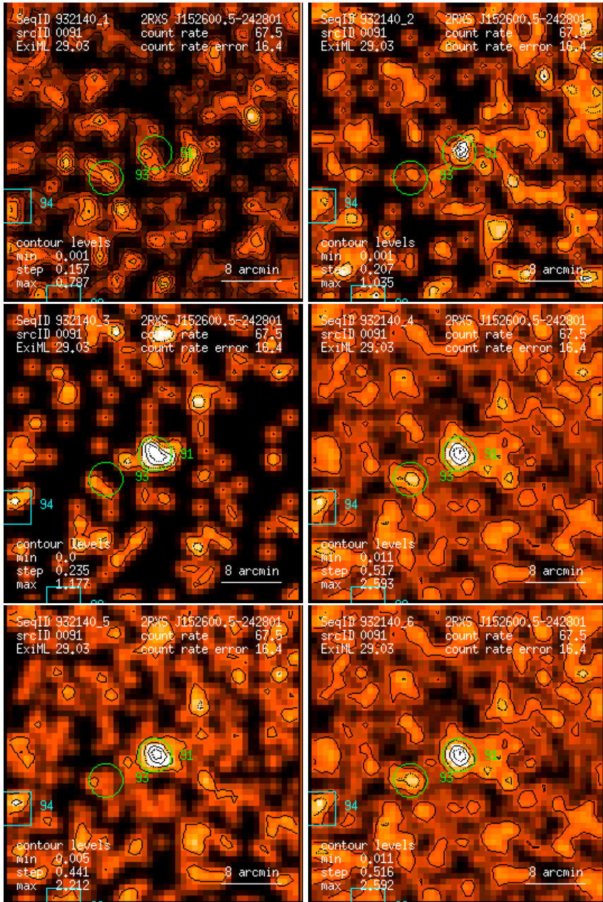
Figure 91: RASS 932140: detection 0091: band rate images, Gaussian filter: (1) PSPC channels 11 – 41, (2) 52 – 90, (3) 91 – 201, (4) 11 – 235, (5) 52 – 201, (6) 11 – 201. Broad band rates in counts/ks. Band rate contour levels in counts/ks/arcmin 2 .
