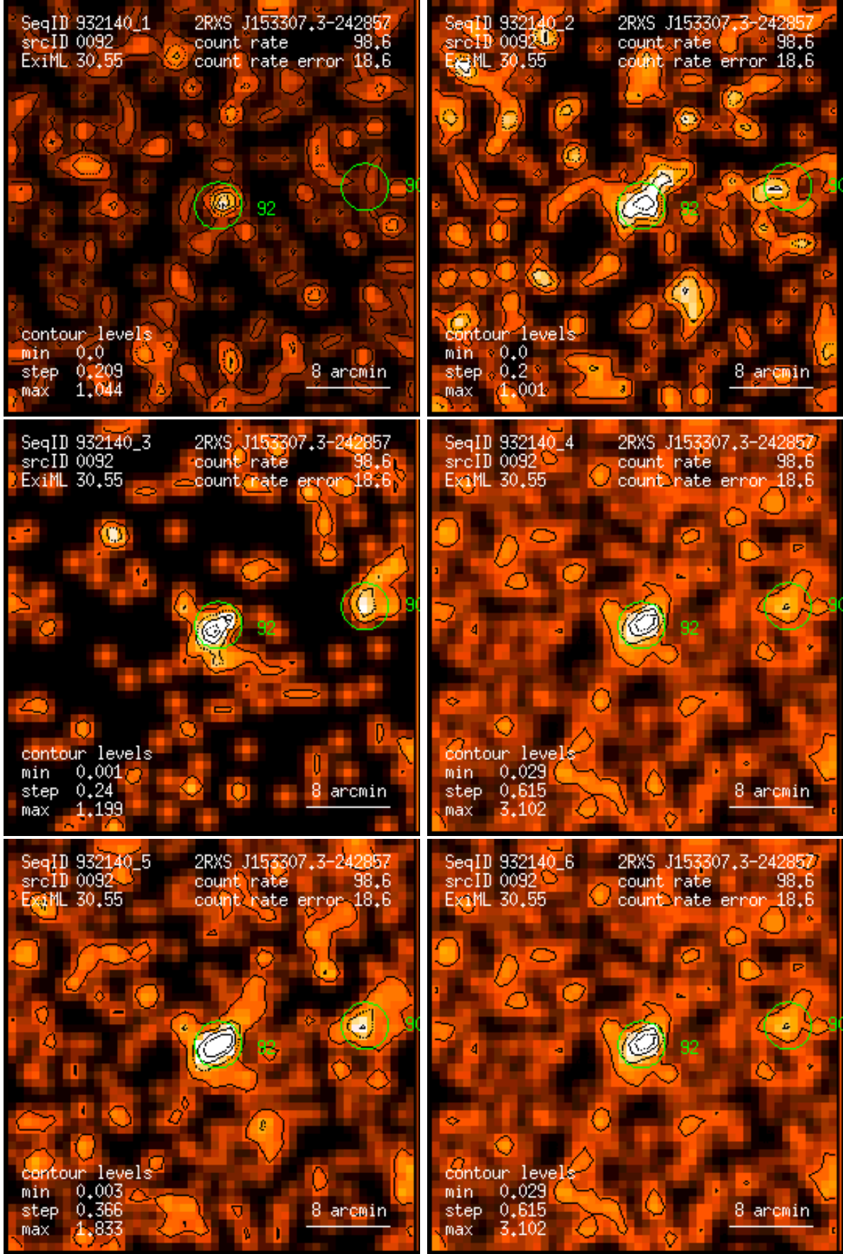
Figure 92: RASS 932140: detection 0092: band rate images, Gaussian filter: (1) PSPC channels 11 – 41, (2) 52 – 90, (3) 91 – 201, (4) 11 – 235, (5) 52 – 201, (6) 11 – 201. Broad band rates in counts/ks. Band rate contour levels in counts/ks/arcmin 2 .
