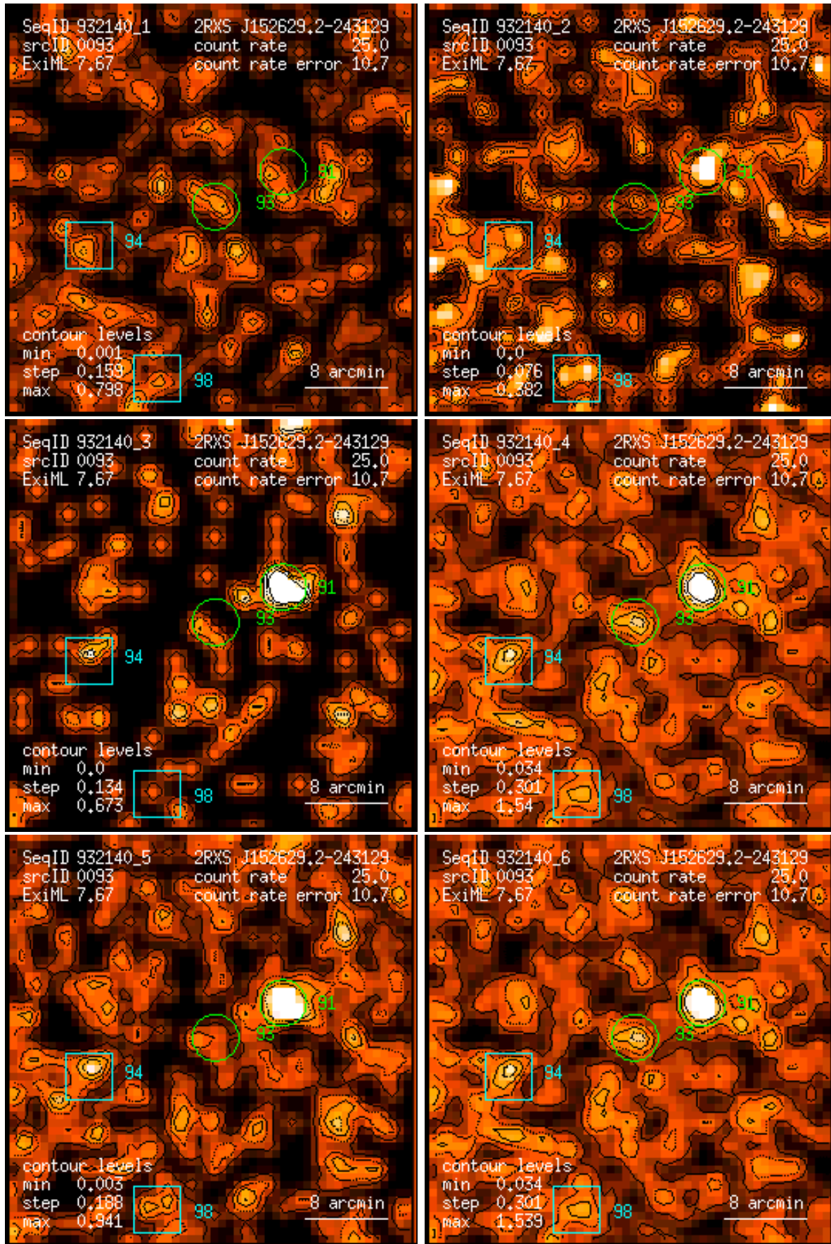
Figure 93: RASS 932140: detection 0093: band rate images, Gaussian filter: (1) PSPC channels 11 – 41, (2) 52 – 90, (3) 91 – 201, (4) 11 – 235, (5) 52 – 201, (6) 11 – 201. Broad band rates in counts/ks. Band rate contour levels in counts/ks/arcmin 2 .
