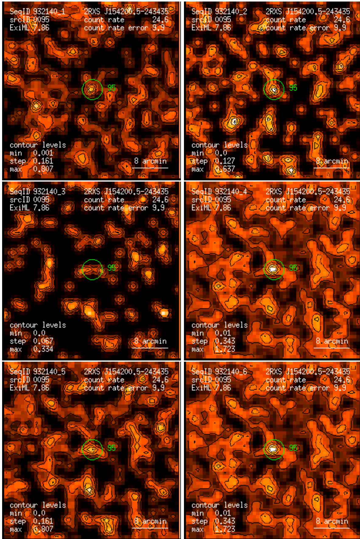
Figure 95: RASS 932140: detection 0095: band rate images, Gaussian filter: (1) PSPC channels 11 – 41, (2) 52 – 90, (3) 91 – 201, (4) 11 – 235, (5) 52 – 201, (6) 11 – 201. Broad band rates in counts/ks. Band rate contour levels in counts/ks/arcmin 2 .
