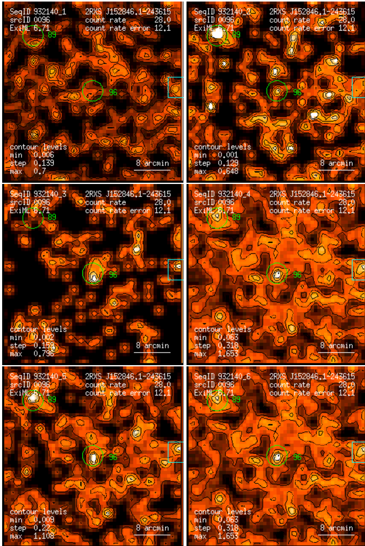
Figure 96: RASS 932140: detection 0096: band rate images, Gaussian filter: (1) PSPC channels 11 – 41, (2) 52 – 90, (3) 91 – 201, (4) 11 – 235, (5) 52 – 201, (6) 11 – 201. Broad band rates in counts/ks. Band rate contour levels in counts/ks/arcmin 2 .
