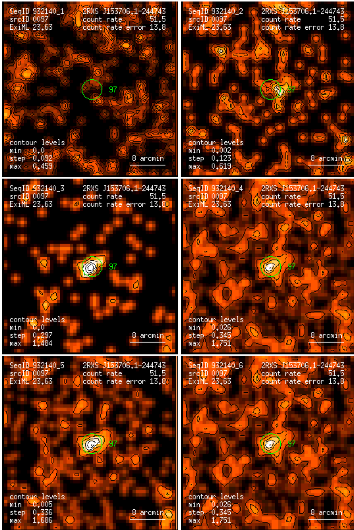
Figure 97: RASS 932140: detection 0097: band rate images, Gaussian filter: (1) PSPC channels 11 – 41, (2) 52 – 90, (3) 91 – 201, (4) 11 – 235, (5) 52 – 201, (6) 11 – 201. Broad band rates in counts/ks. Band rate contour levels in counts/ks/arcmin 2 .
