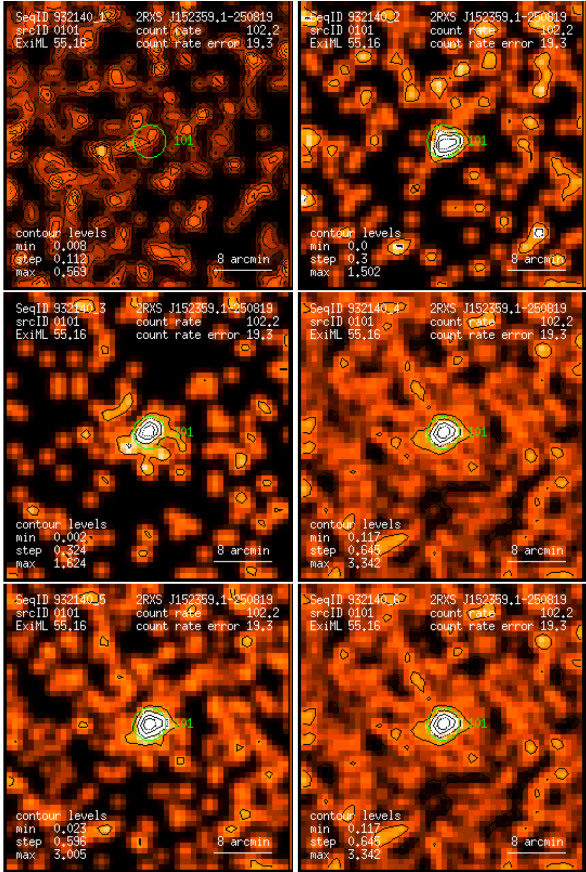
Figure 101: RASS 932140: detection 0101: band rate images, Gaussian filter: (1) PSPC channels 11 – 41, (2) 52 – 90, (3) 91 – 201, (4) 11 – 235, (5) 52 – 201, (6) 11 – 201. Broad band rates in counts/ks. Band rate contour levels in counts/ks/arcmin 2 .
