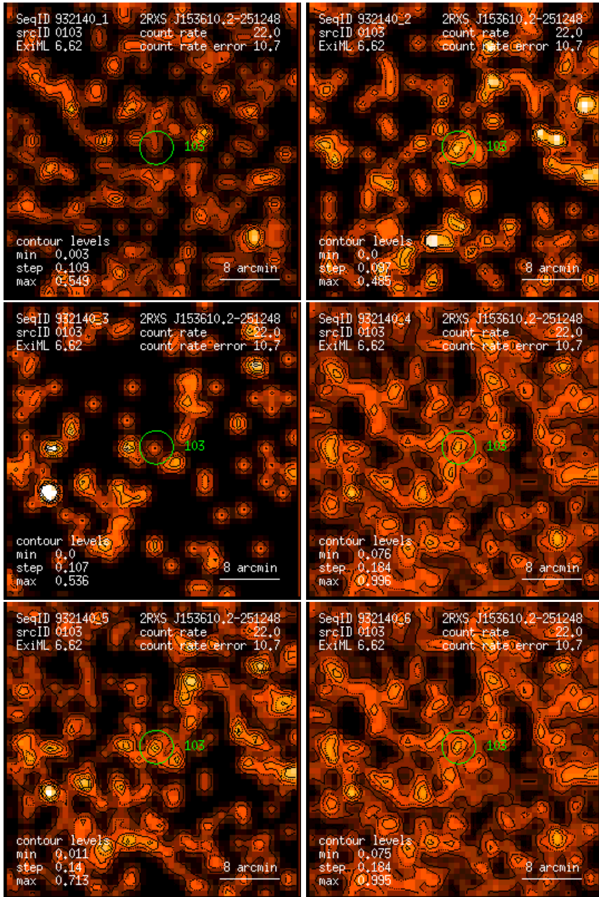
Figure 103: RASS 932140: detection 0103: band rate images, Gaussian filter: (1) PSPC channels 11 – 41, (2) 52 – 90, (3) 91 – 201, (4) 11 – 235, (5) 52 – 201, (6) 11 – 201. Broad band rates in counts/ks. Band rate contour levels in counts/ks/arcmin 2 .
