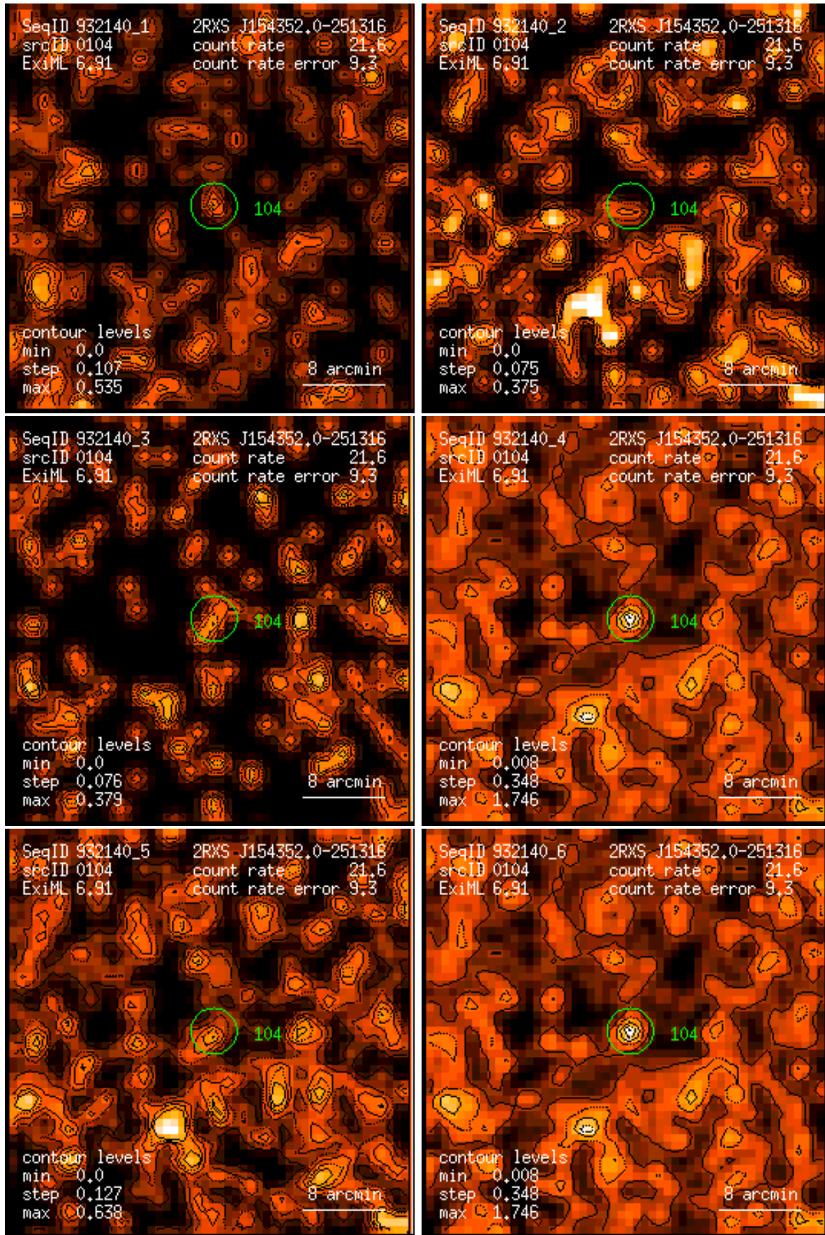
Figure 104: RASS 932140: detection 0104: band rate images, Gaussian filter: (1) PSPC channels 11 – 41, (2) 52 – 90, (3) 91 – 201, (4) 11 – 235, (5) 52 – 201, (6) 11 – 201. Broad band rates in counts/ks. Band rate contour levels in counts/ks/arcmin 2 .
