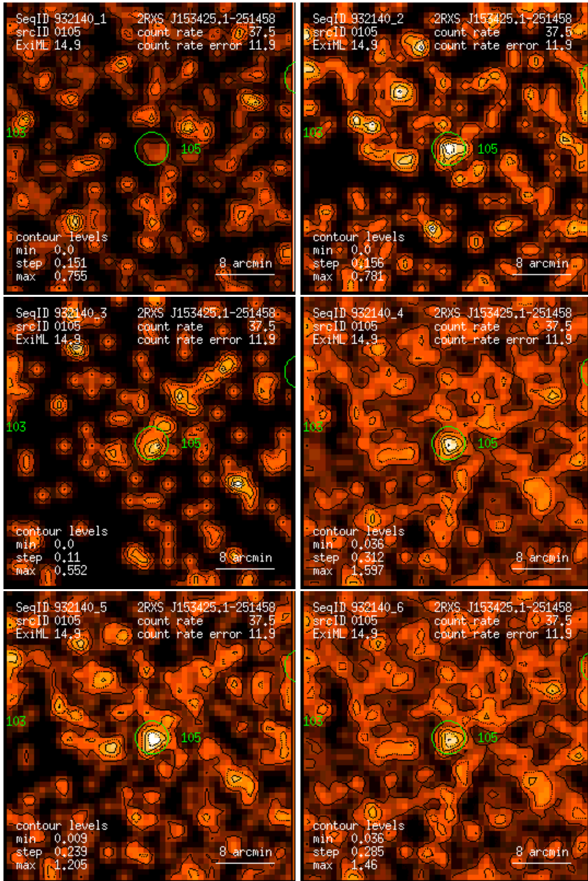
Figure 105: RASS 932140: detection 0105: band rate images, Gaussian filter: (1) PSPC channels 11 – 41, (2) 52 – 90, (3) 91 – 201, (4) 11 – 235, (5) 52 – 201, (6) 11 – 201. Broad band rates in counts/ks. Band rate contour levels in counts/ks/arcmin 2 .
