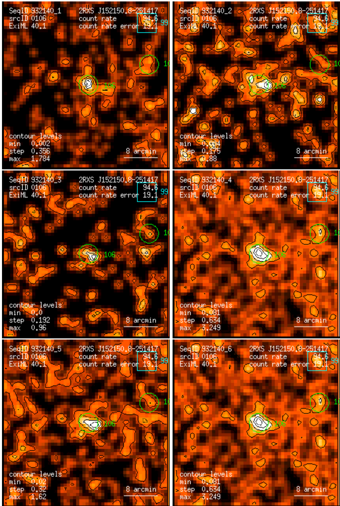
Figure 106: RASS 932140: detection 0106: band rate images, Gaussian filter: (1) PSPC channels 11 – 41, (2) 52 – 90, (3) 91 – 201, (4) 11 – 235, (5) 52 – 201, (6) 11 – 201. Broad band rates in counts/ks. Band rate contour levels in counts/ks/arcmin 2 .
