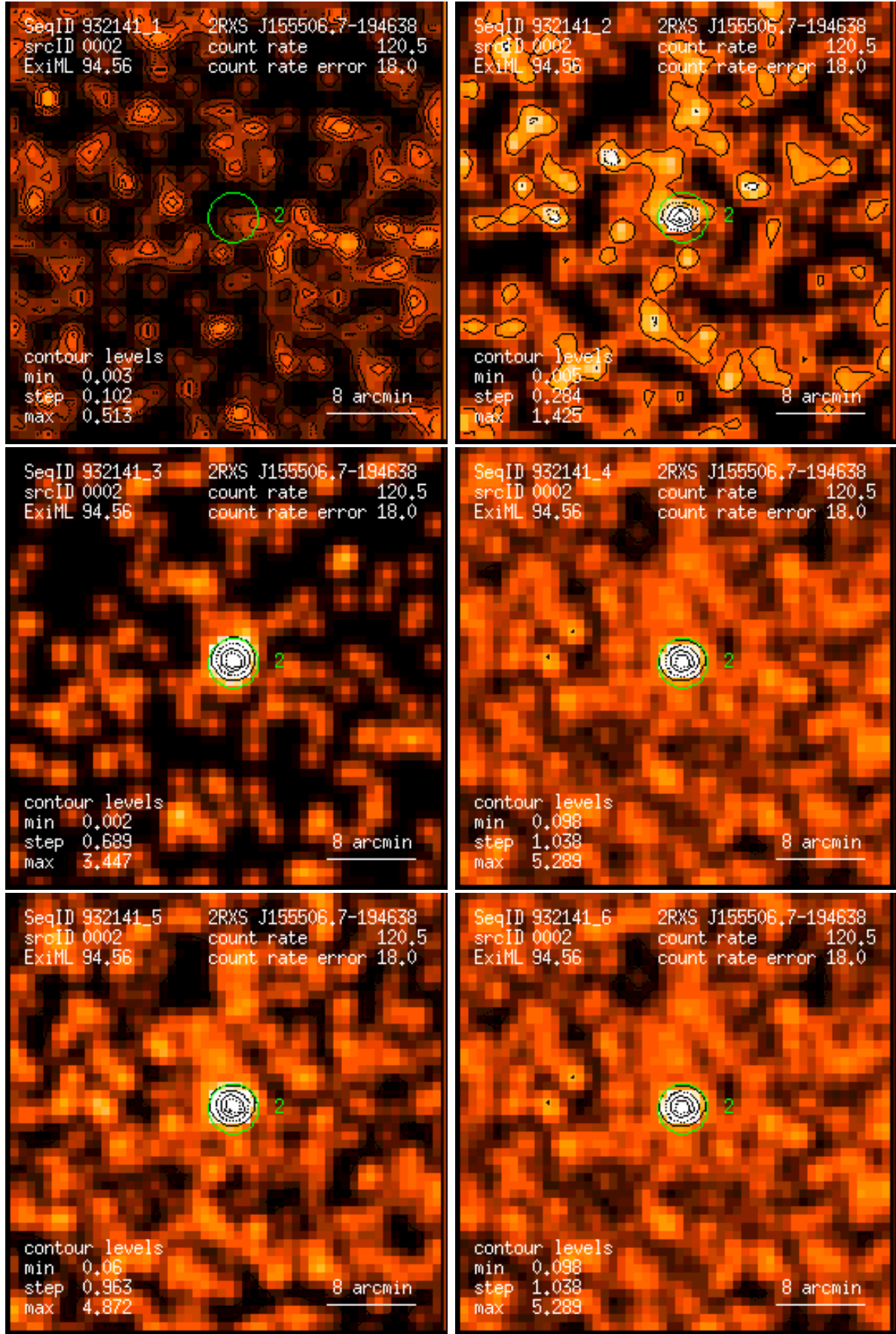
Figure 2: RASS 932141: detection 0002: band rate images, Gaussian filter: (1) PSPC channels 11 – 41, (2) 52 – 90, (3) 91 – 201, (4) 11 – 235, (5) 52 – 201, (6) 11 – 201. Broad band rates in counts/ks. Band rate contour levels in counts/ks/arcmin 2 .
