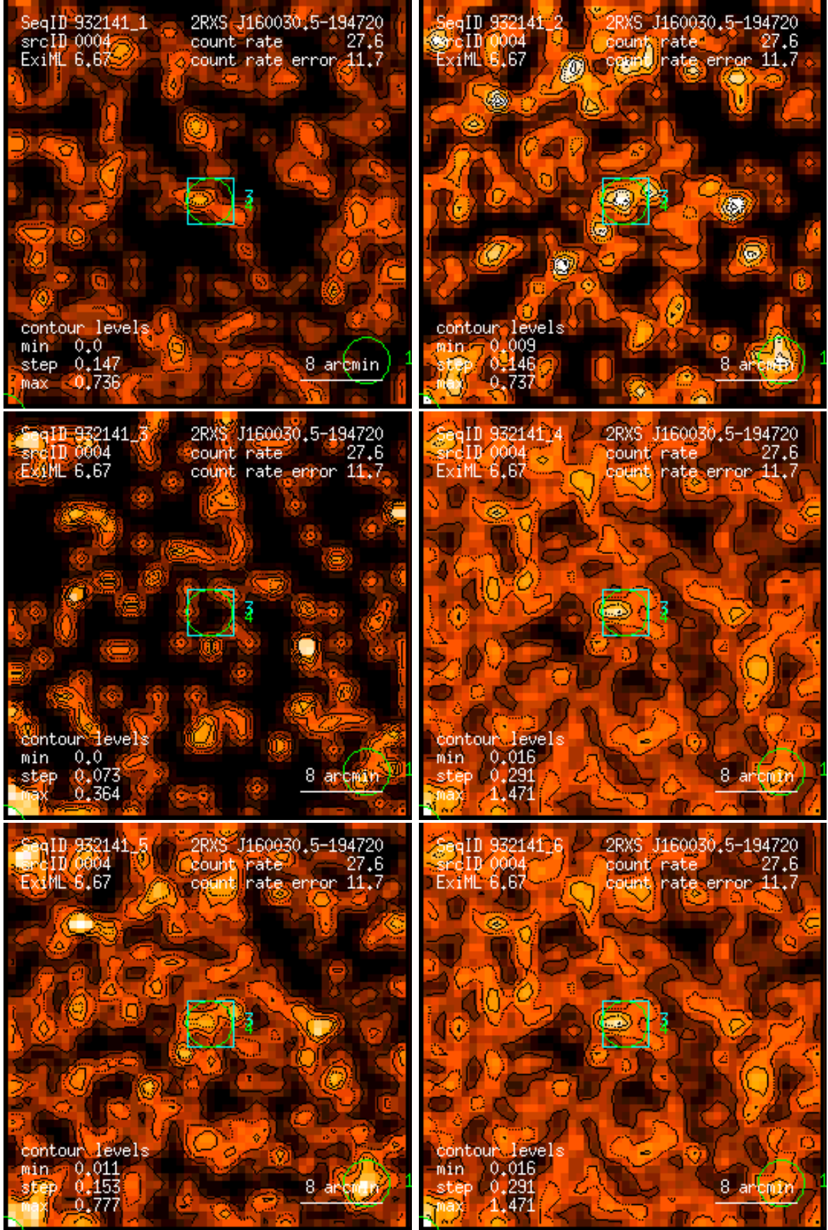
Figure 4: RASS 932141: detection 0004: band rate images, Gaussian filter: (1) PSPC channels 11 – 41, (2) 52 – 90, (3) 91 – 201, (4) 11 – 235, (5) 52 – 201, (6) 11 – 201. Broad band rates in counts/ks. Band rate contour levels in counts/ks/arcmin 2 .
