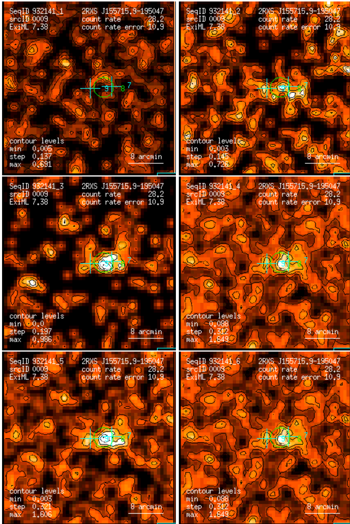
Figure 9: RASS 932141: detection 0009: band rate images, Gaussian filter: (1) PSPC channels 11 – 41, (2) 52 – 90, (3) 91 – 201, (4) 11 – 235, (5) 52 – 201, (6) 11 – 201. Broad band rates in counts/ks. Band rate contour levels in counts/ks/arcmin 2 .
