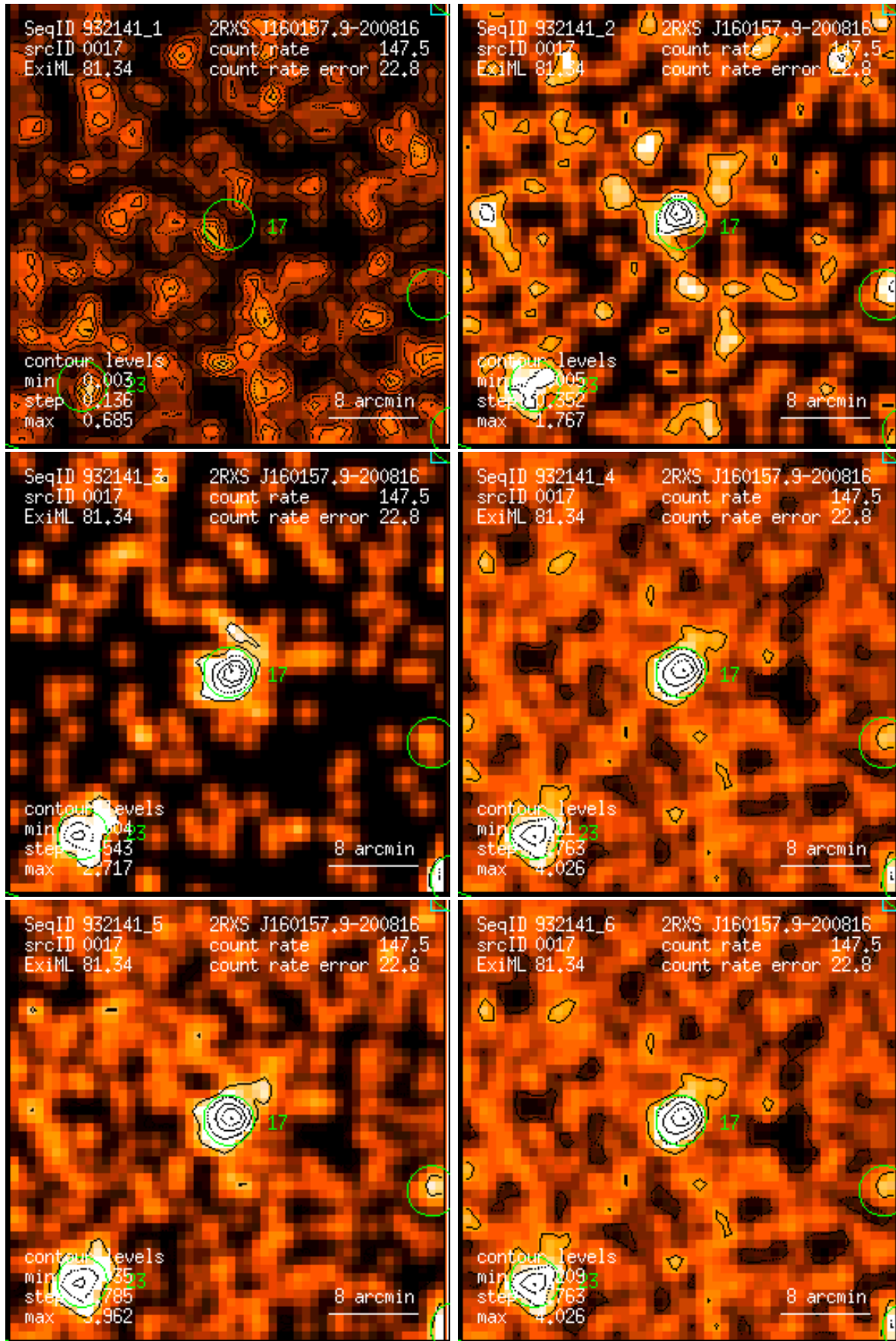
Figure 17: RASS 932141: detection 0017: band rate images, Gaussian filter: (1) PSPC channels 11 – 41, (2) 52 – 90, (3) 91 – 201, (4) 11 – 235, (5) 52 – 201, (6) 11 – 201. Broad band rates in counts/ks. Band rate contour levels in counts/ks/arcmin 2 .
