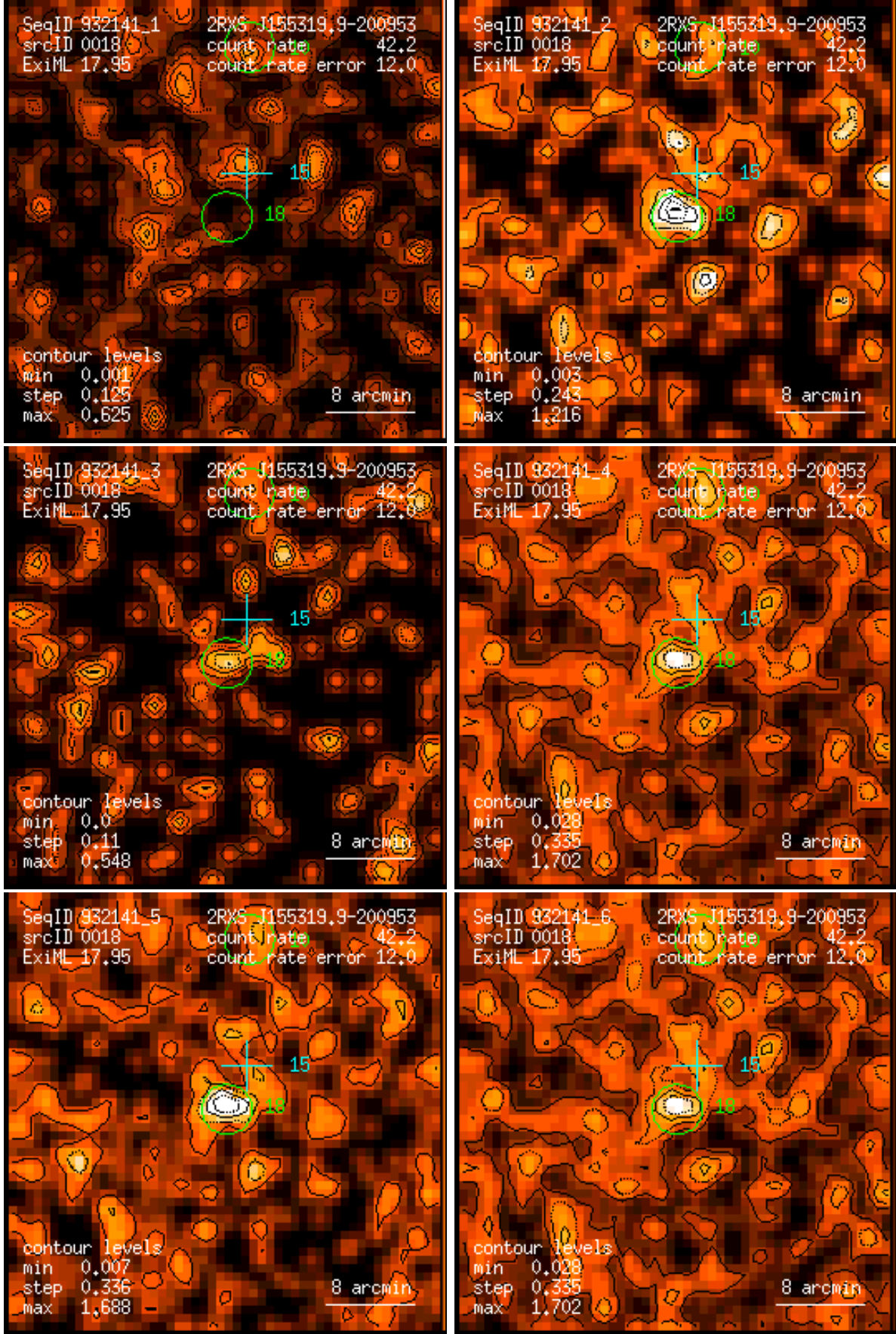
Figure 18: RASS 932141: detection 0018: band rate images, Gaussian filter: (1) PSPC channels 11 – 41, (2) 52 – 90, (3) 91 – 201, (4) 11 – 235, (5) 52 – 201, (6) 11 – 201. Broad band rates in counts/ks. Band rate contour levels in counts/ks/arcmin 2 .
