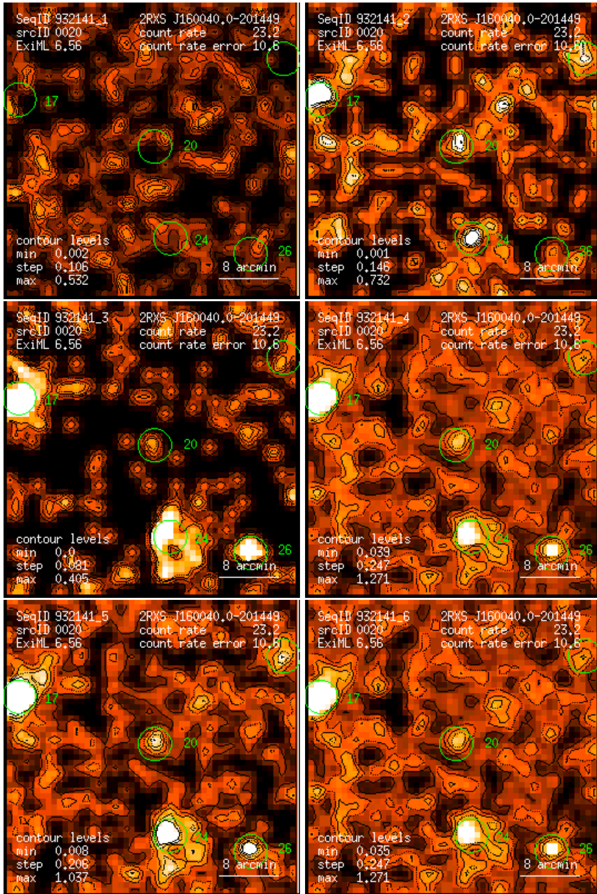
Figure 20: RASS 932141: detection 0020: band rate images, Gaussian filter: (1) PSPC channels 11 – 41, (2) 52 – 90, (3) 91 – 201, (4) 11 – 235, (5) 52 – 201, (6) 11 – 201. Broad band rates in counts/ks. Band rate contour levels in counts/ks/arcmin 2 .
