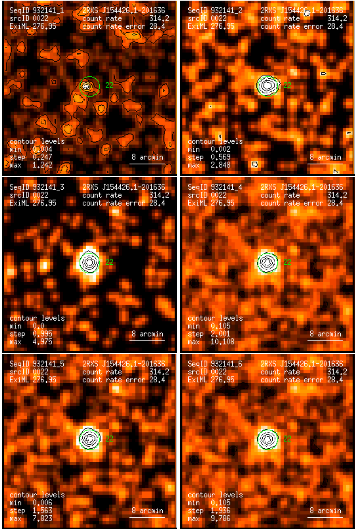
Figure 22: RASS 932141: detection 0022: band rate images, Gaussian filter: (1) PSPC channels 11 – 41, (2) 52 – 90, (3) 91 – 201, (4) 11 – 235, (5) 52 – 201, (6) 11 – 201. Broad band rates in counts/ks. Band rate contour levels in counts/ks/arcmin 2 .
